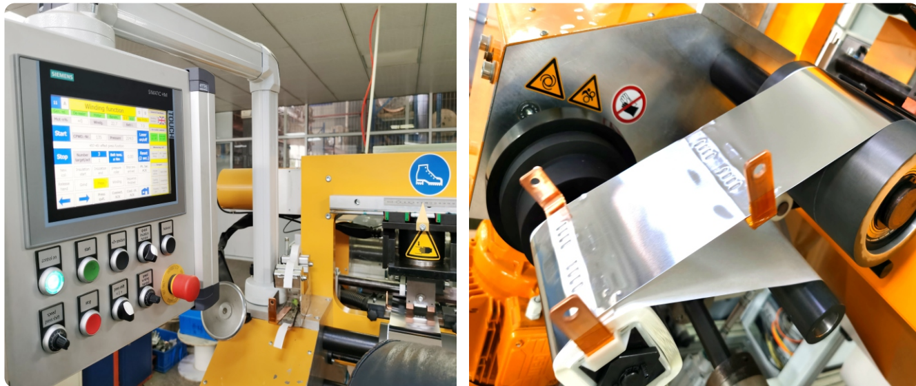
Copper & Aluminum cold pressure welding
